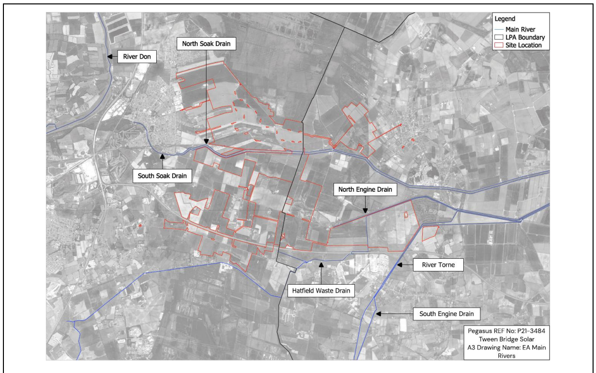
Figure 3.3 – Main Rivers
